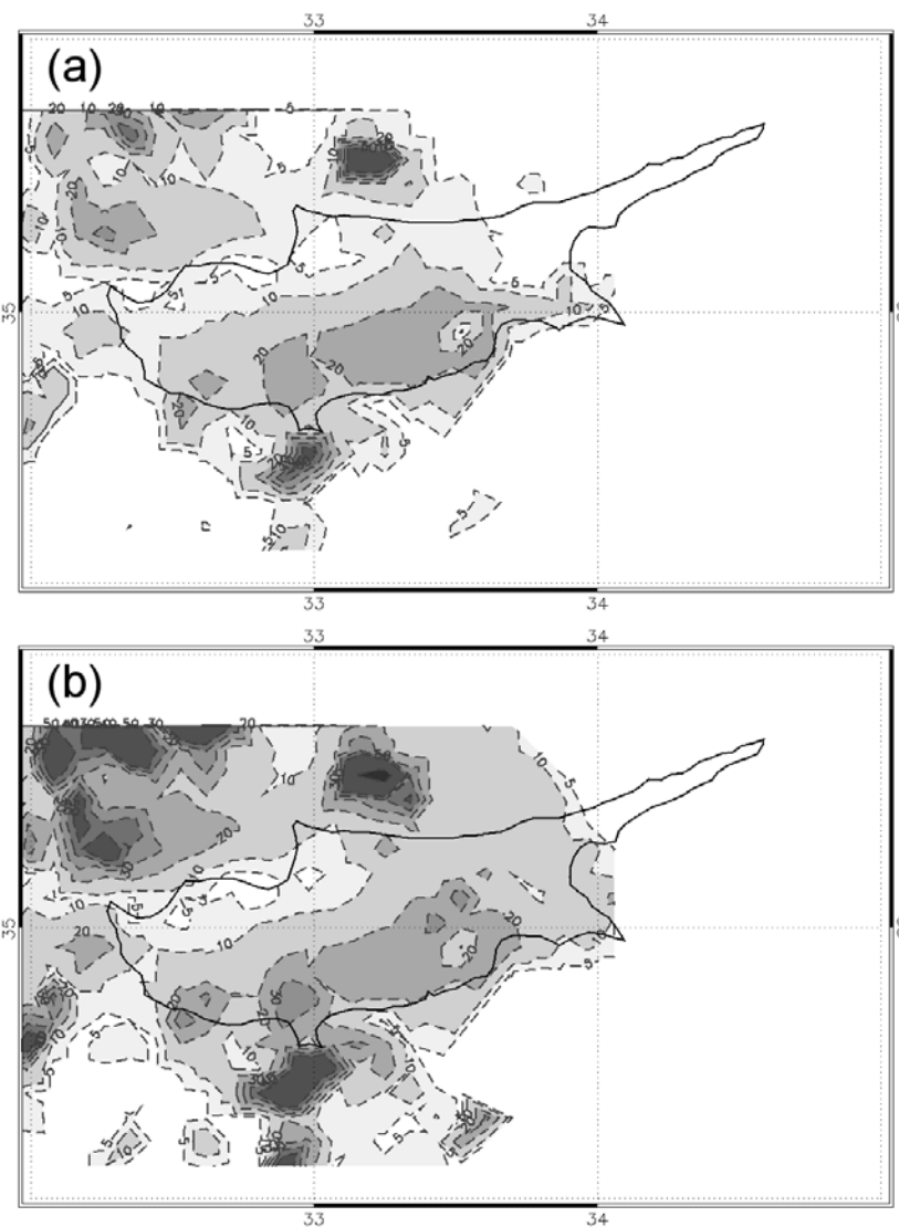
Fig. 8. Contours (in mm) of radar-rain gauge composite using OGRD (a) and RGRD (b). Precipitation is 24-h accumulated from 0600 UTC 5 March to 0600 UTC 6 March 2003.
