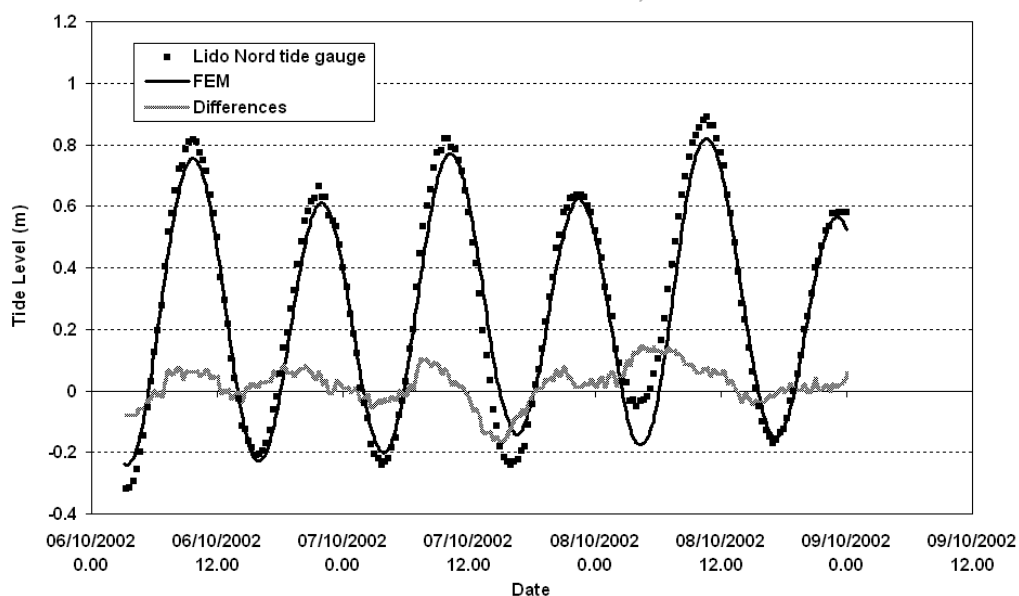
MEDIUM-HIGH TIDE EVENT — VENICE, 6-8 OCT. 2002
